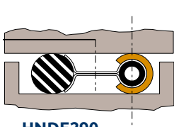
HNDE290 Leak check - Insert Gas Purge
