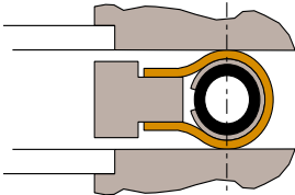
HN208 Raised face flange - ANSI B16.5
