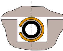
HN200 Groove Assembly
