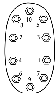
Noncircular Multibolt
