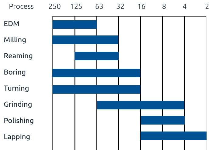
Approximate Roughness Average, RMS
